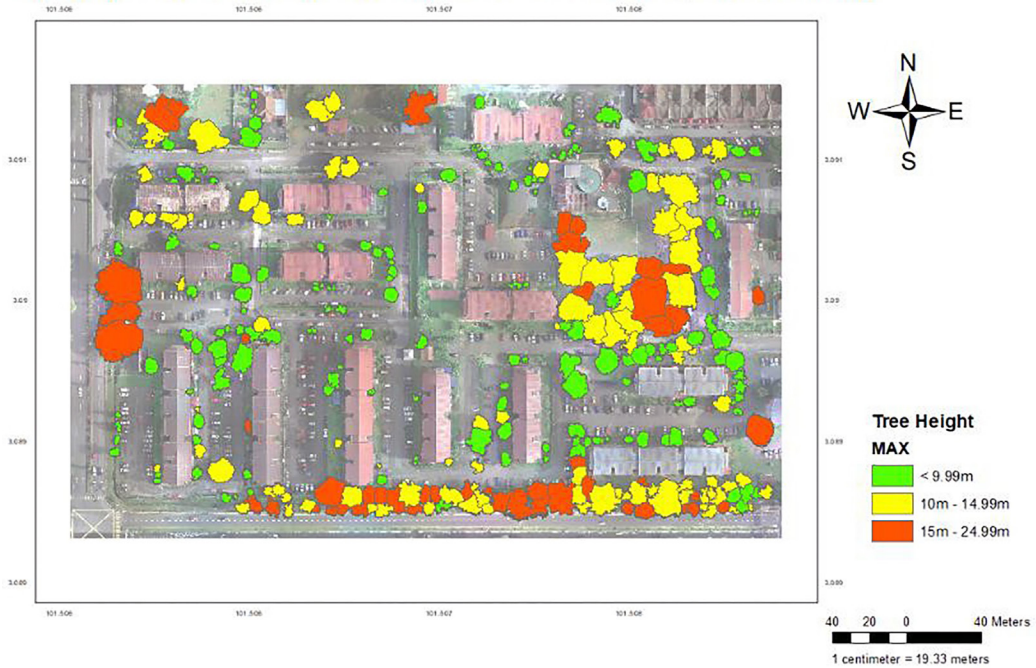
Figure 10. Individual tree height map
