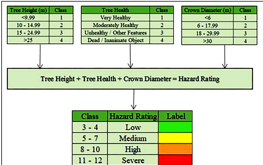
Figure 4. Classification of hazard rating assessment
