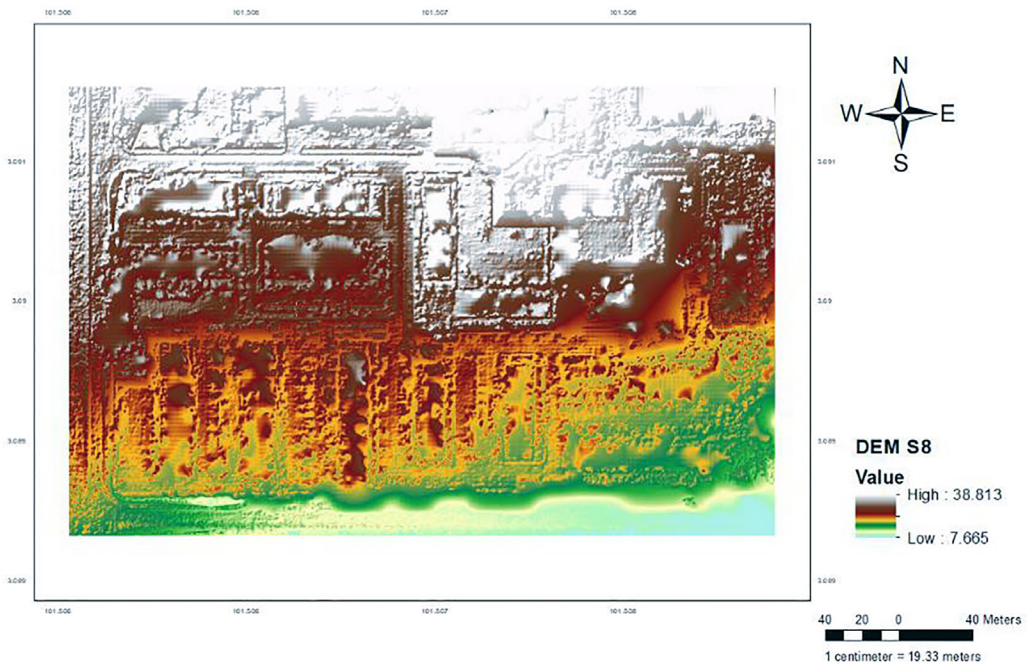
Figure 5. Digital elevation model
