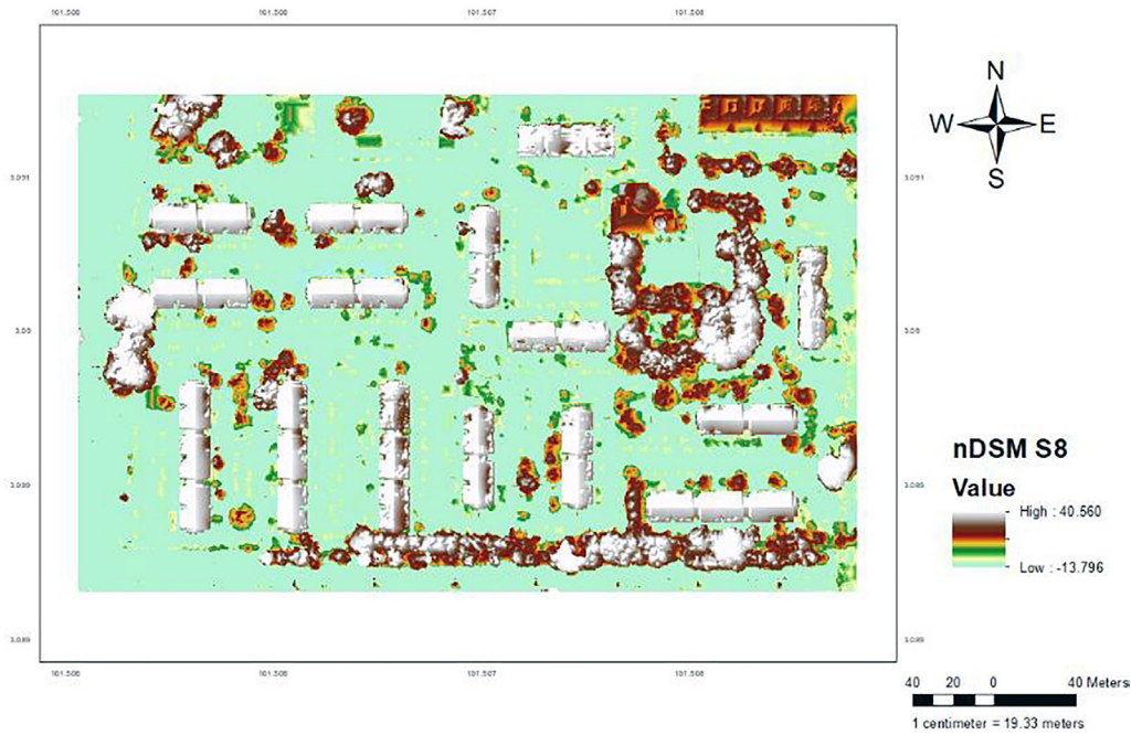
Figure 7. Normalized digital surface model
