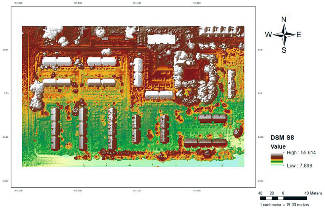
Figure 6. Digital surface model
