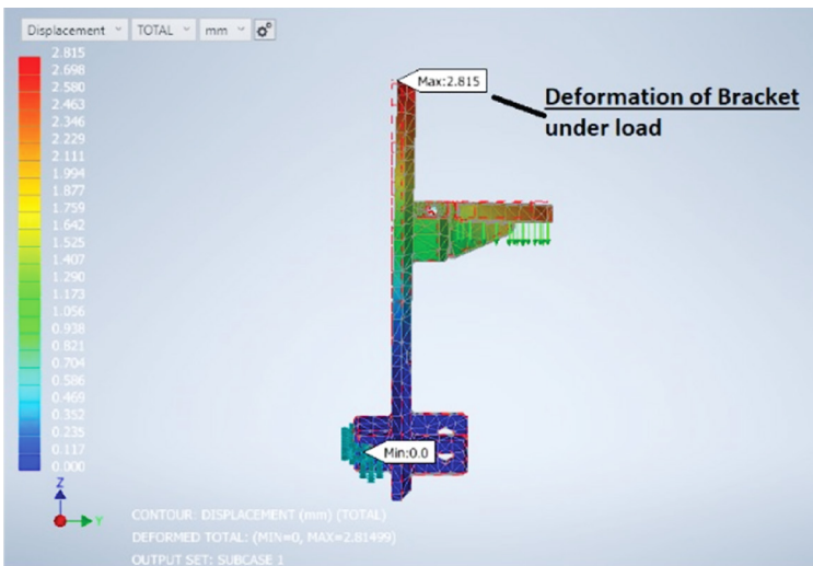
Figure 5. Contour displacement of footrest bracket deformed
