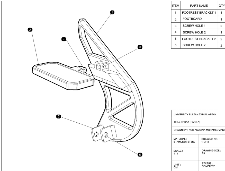
Figure 1. Exploded view of P.Jacq™
