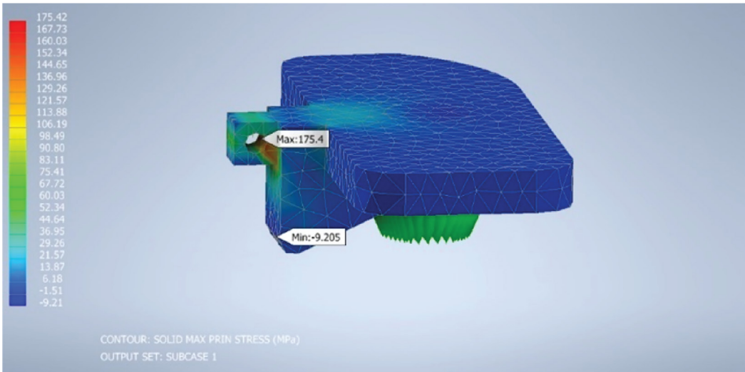
Figure 4. Comparison of screw hole 2 on P.Jacq™ 2021 model
